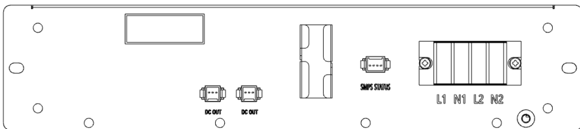
Figure 2-13: Front View of SMPS Assembly Type B, 1-Phase Input
