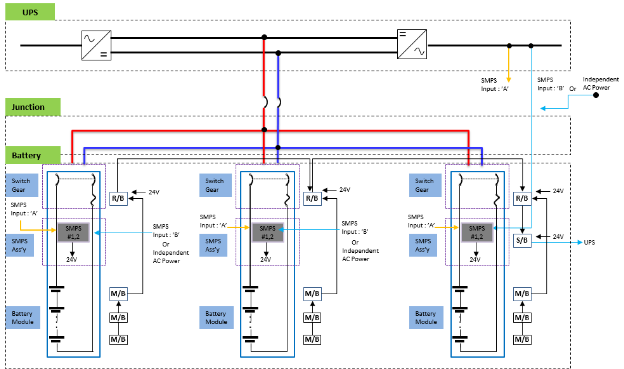
Figure 2-15: System Block Diagram
