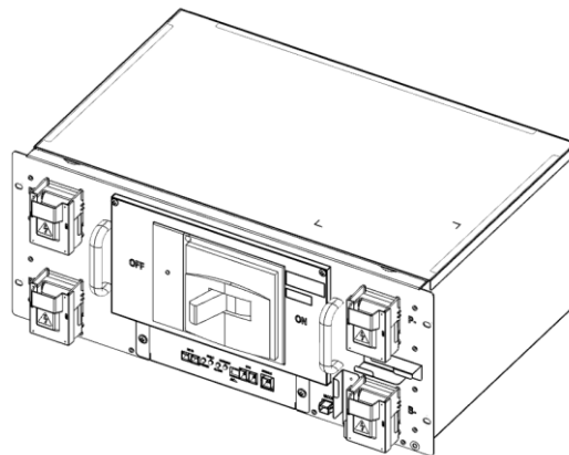
Figure 2-3: BCU
