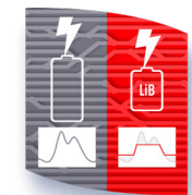
Expanded Functionality
